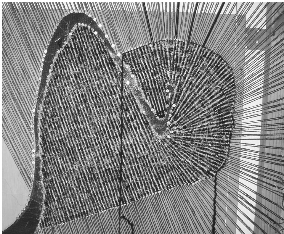
Włodzimierz Cygan, Loom setup for interior opening and diverging warps
